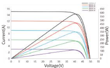
I-V/P-V Curve at Different Irradiation SSA-66HD-610N
