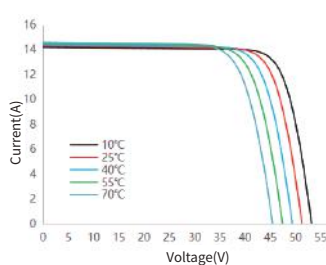
I-V Curve at Different Temperature SS8-72HD-575N
