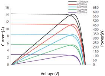
I-V/P-V Curve at Different Irradiation SS8-72HD-575N
