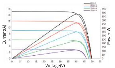
I-V/P-V Curve at Different Irradiation SSA-66HD-610N
