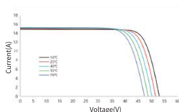
I-V Curve at Different Temperature SSA-66HD-610N
