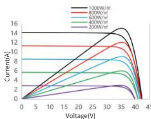
I-V/P-V Curve at Different Irradiation SS8-60HDB-470N
