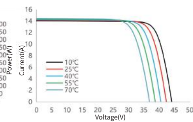
I-V Curve at Different Temperature SS8-60HDB-470N
