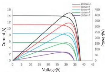
I-V/P-V Curve at Different Irradiation SS8-54HD-420N
