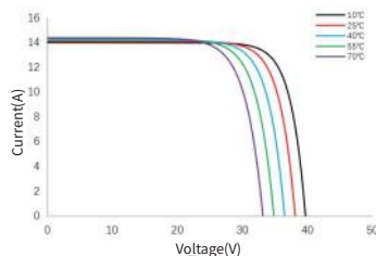
I-V Curve at Different Temperature SS8-54HD-420N
