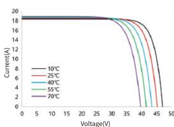
I-V Curve at Different Temperature SS8-66HD-505M
