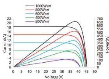
I-V/P-V Curve at Different Irradiation SS8-66HD-505M
