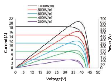
I-V/P-V Curve at Different Irradiation SS9-66HS -660M
