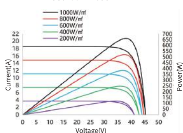
I-V/P-V Curve at Different Irradiation SS9-66HD-655M
