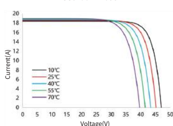
I-V Curve at Different Temperature SS9-66HD-655M
