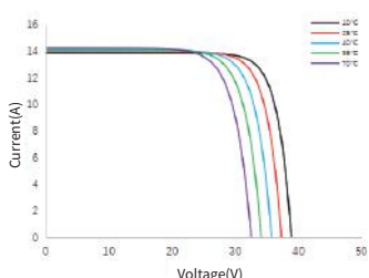
I-V Curve at Different Temperature SS8-54HSB -400M
