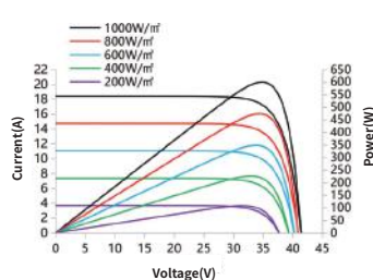
I-V/P-V Curve at Different Irradiation SS9-60HS -600M
