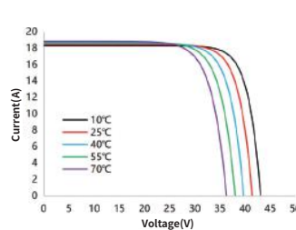
I-V Curve at Different Temperature SS9-60HS -600M
