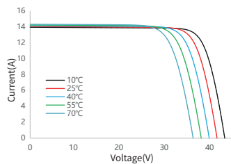
I-V Curve at Different Temperature SS8-60HSB-450M
