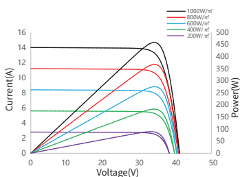
I-V/P-V Curve at Different Irradiation SS8-60HSB-450M
